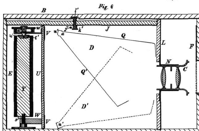
PIVOTED DROP SHUTTER of Eastman's first camera in cross section. When button I' on top of camera is turned, shutter QQ' drops from D to D' ; after exposure is returned to D by a knob on side of the camera, not shown in drawing.
